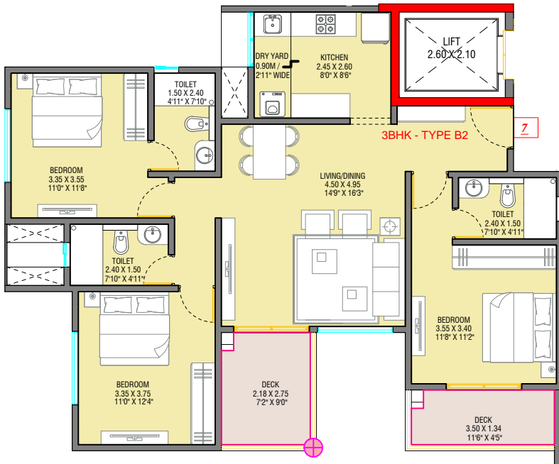
EVEN FLOOR 3 BHK TYPE B - UNIT 4 / 7
