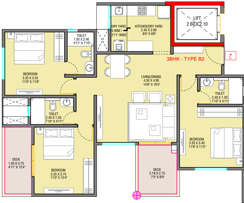
ODD FLOOR 3 BHK TYPE B - UNIT 4 / 7
